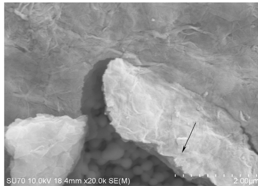
(b) surface image of composite NF membrane (1 layer)
